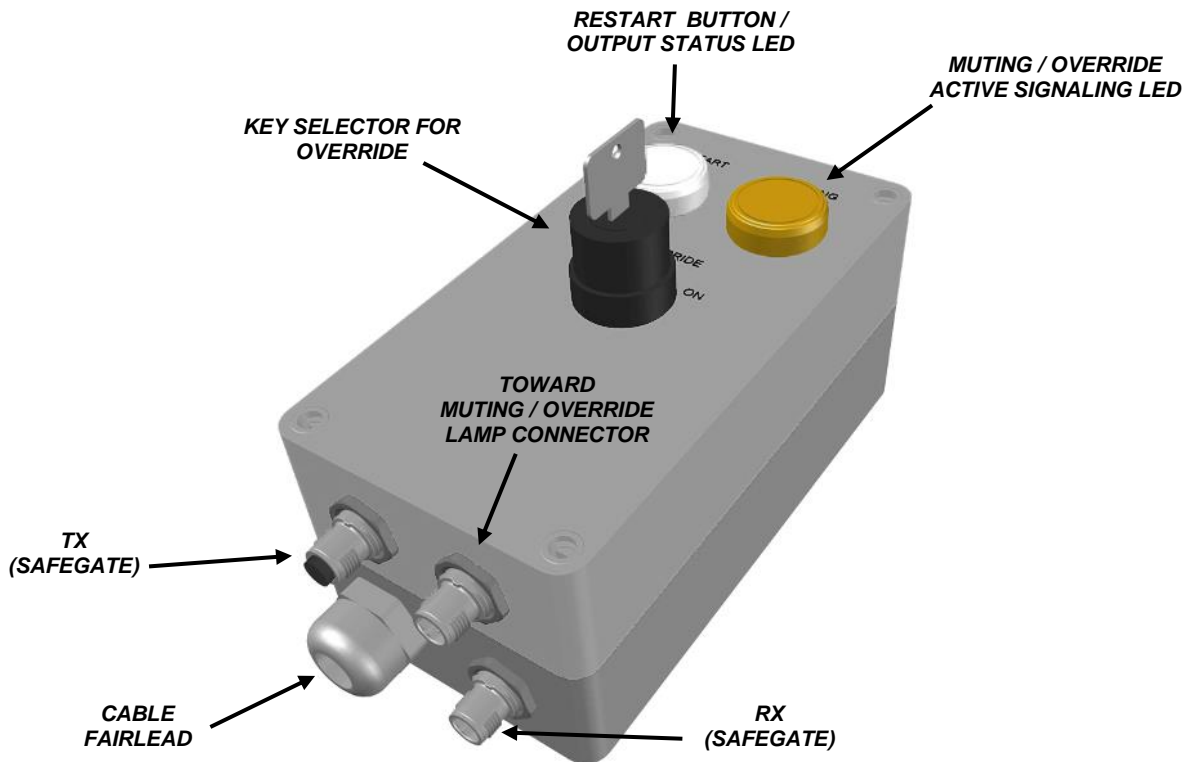
Figure 4 - M SGO BOX PLUS – Connections and signals
