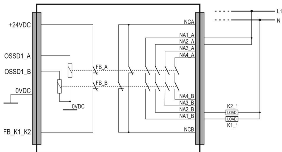
Figure 6 – M SGO BOX PLUS connection sample
